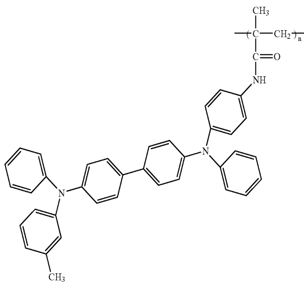
TPD-MAA
