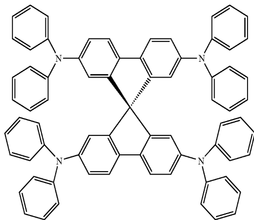
spiro-TPD
