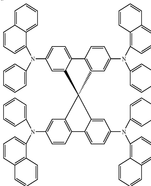
spiro-NPD
