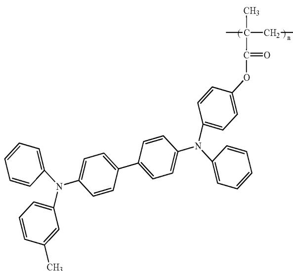
TPD-PMMA
