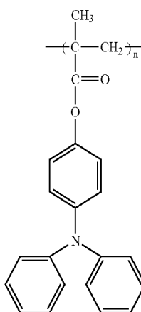
TPA-PMMA
